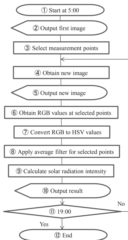
Fig. 5 Flow chart of developed system.
