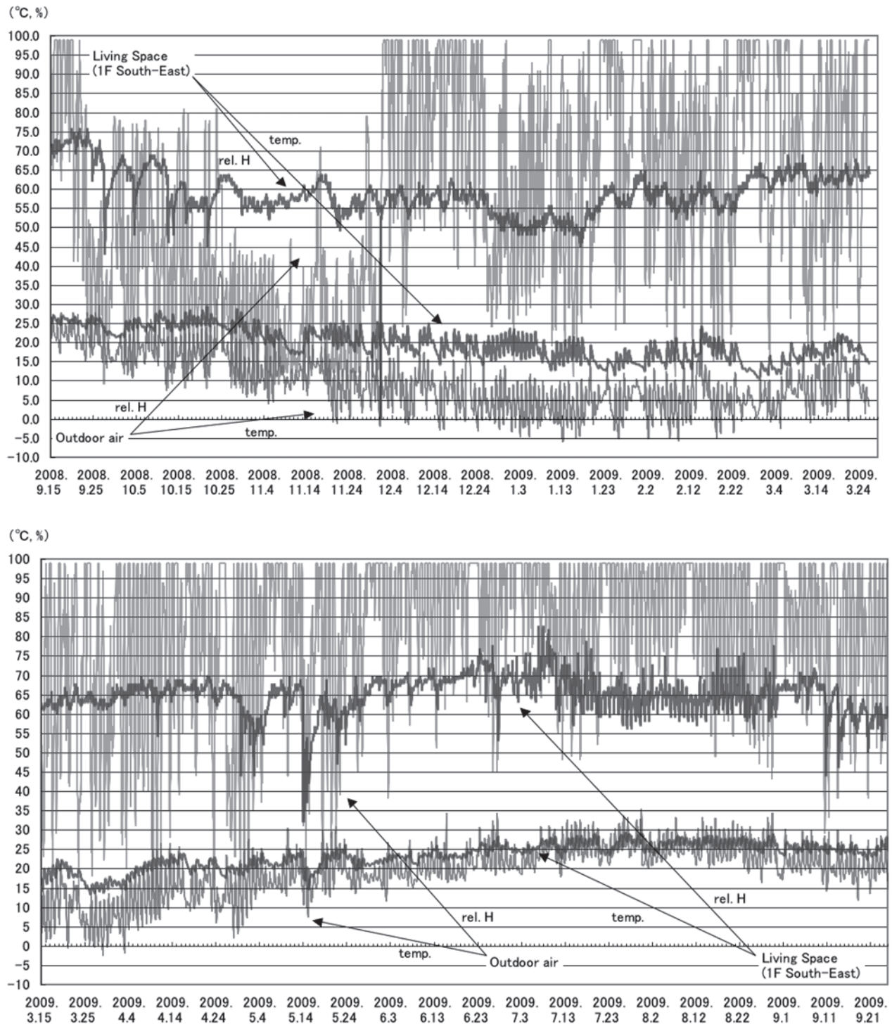
Fig. 5 Temperature (temp.) and relative humidity (rel. H) of living space (1F South-east part) of the experimental house and outdoor air, through a year. Upper; autumn and winter, lower; spring and summer.
