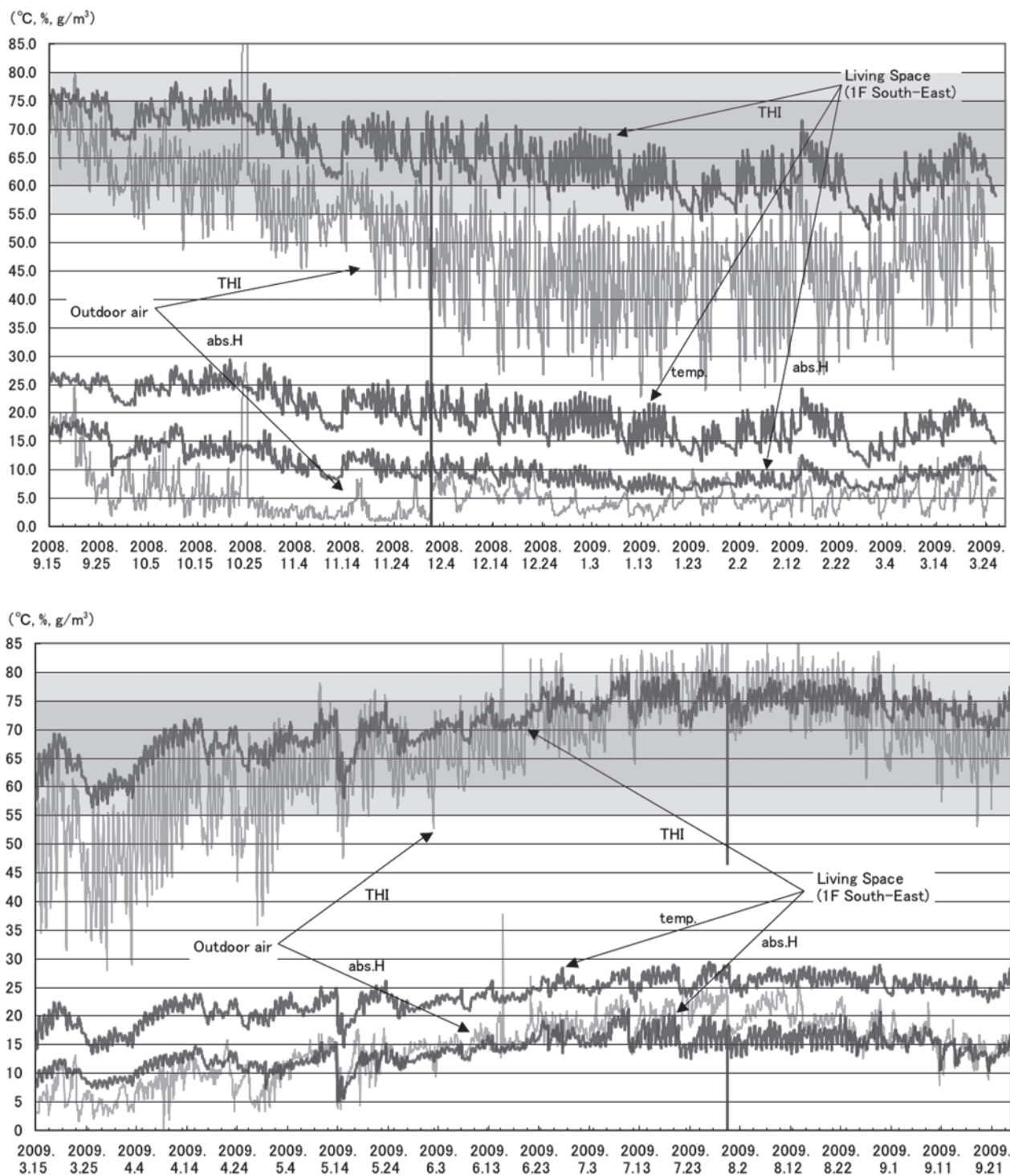
Fig. 6 Temperature humidity index (THI), temperature (temp.) and absolute humidity (abs. H) of living space (1F South-east part) of the experimental house and outdoor air, through a year. Upper; autumn and winter, lower; spring and summer.
