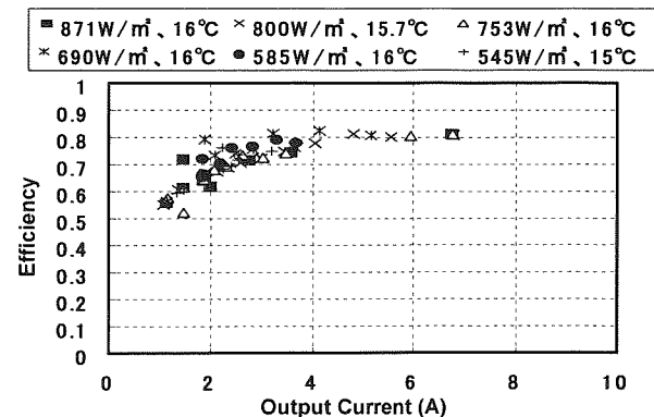
Fig.6 Electric power conversion efficiency of an inverter for different output current.
