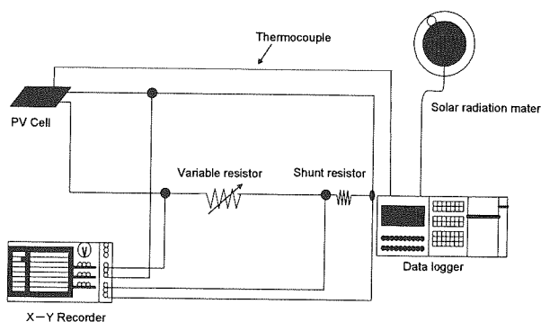
Fig.2 Test circuit for PV cell characteristics.
