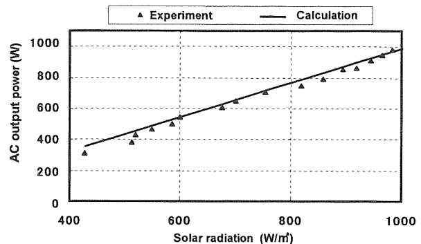
Fig.10 Maximum power against the solar radiation
