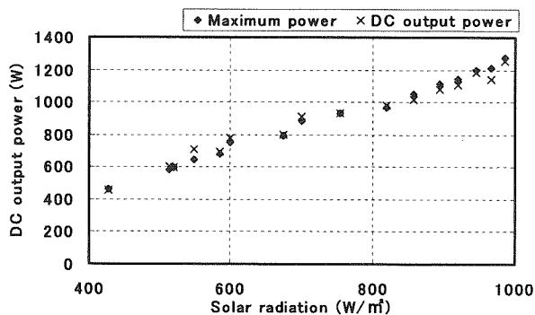
Fig.8 Comparison between Maximum output and DC output power
