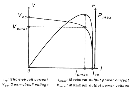
Fig.1 I-V, I-P characteristics of a PV cell.
