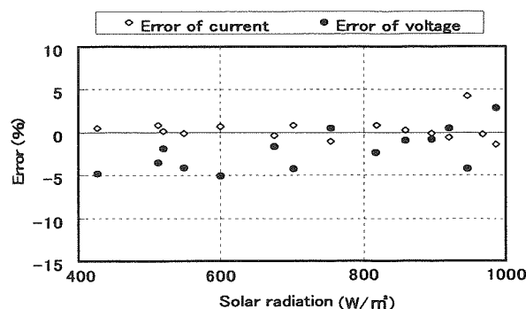
Fig.13 The error of Current and Voltage by formula to output measured in the experiment.
