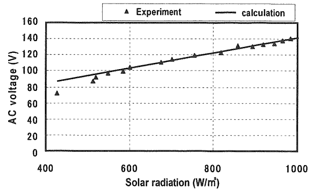
Fig.9 Maximum AC voltage against the solar radiation.
