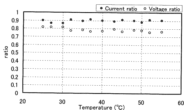
Fig.4 Current ratio and Voltage ratio with the change of temperature.
