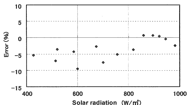
Fig.12 The error of output by formula to output measured in the experiment.
