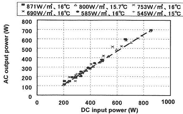
Fig.7 Relation between the output and the input.
