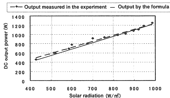
Fig.11 Maximum power against the solar radiation.
