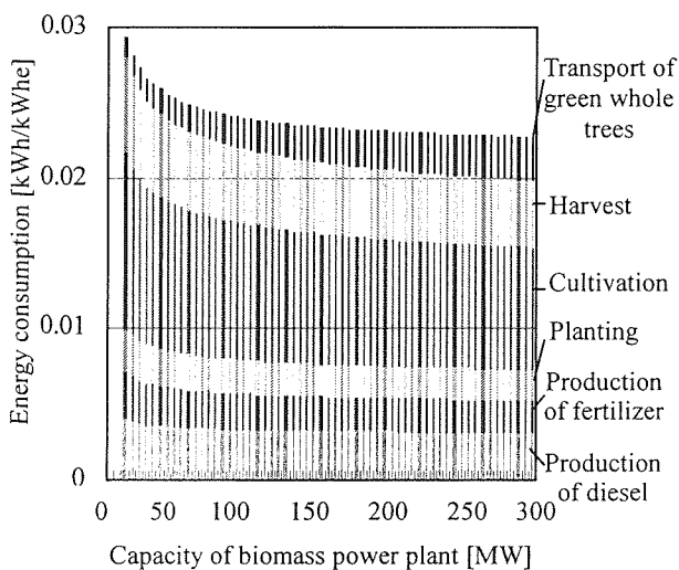
Fig. 9 Items of primary energy consumption (Type of system: BIG/CCa)
