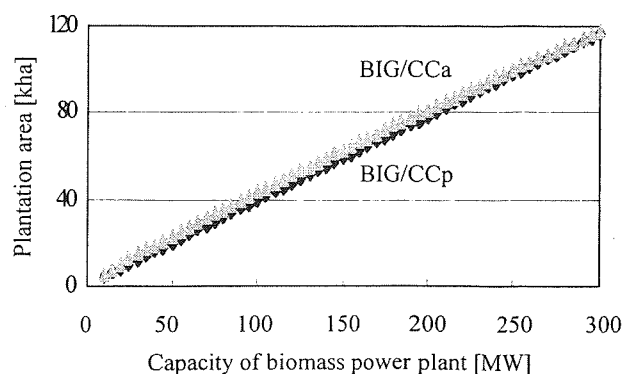
Fig.6 Plantation area required for biomass power generation
